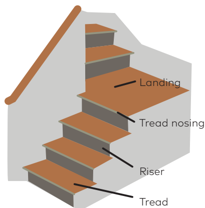
Two-flight staircase with landing
